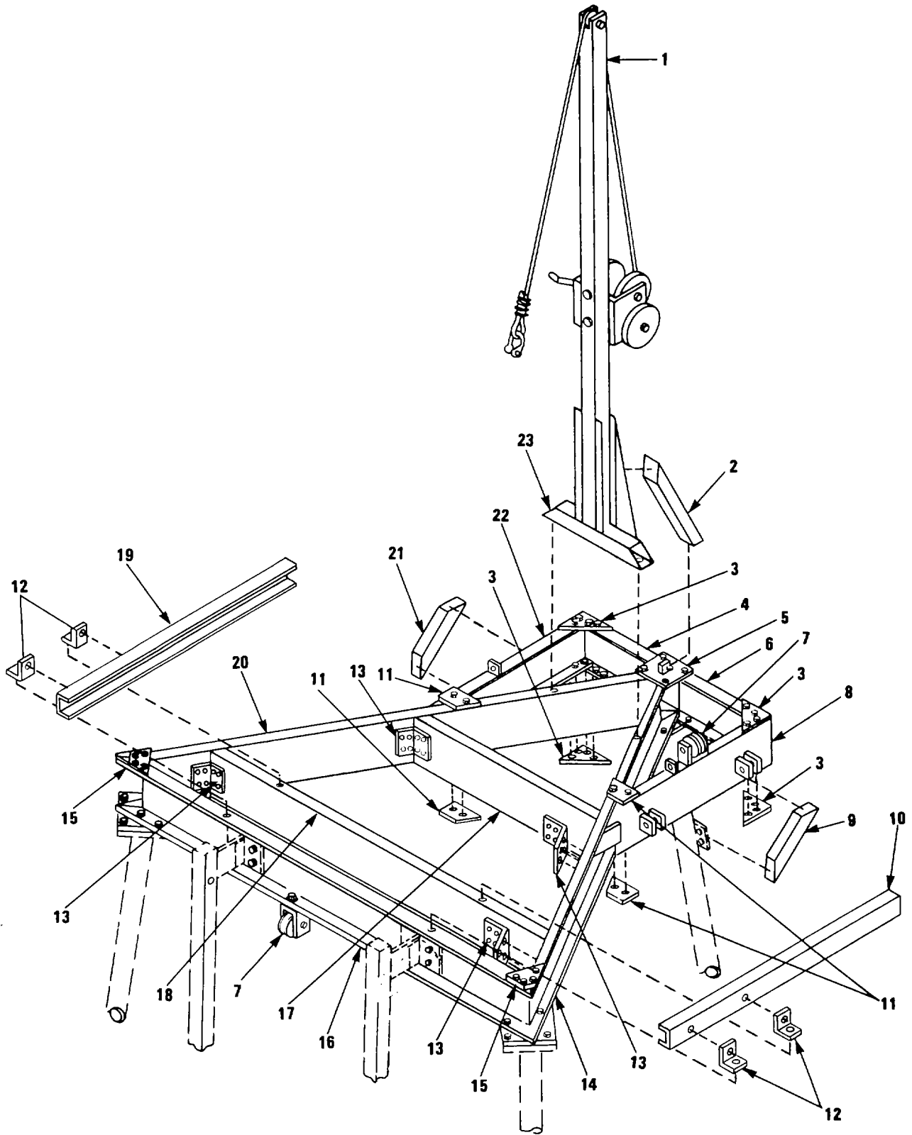
Figure E-6. Tower Adapter Installation (Sheet 1 of 4)
