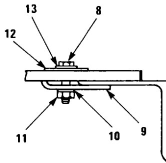
TYPE A GRATING CLAMP ASSEMBLY
