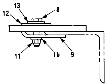
TYPE A GRATING CLAMP ASSEMBLY
